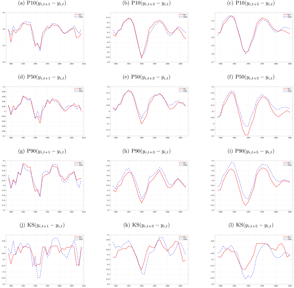
Figure A.1: Sweden: Pre-Government Income Fit
